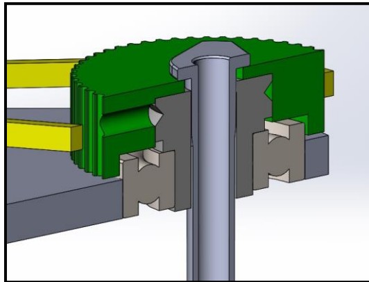
New (large) sample-tube pulley placed over existing pulley
